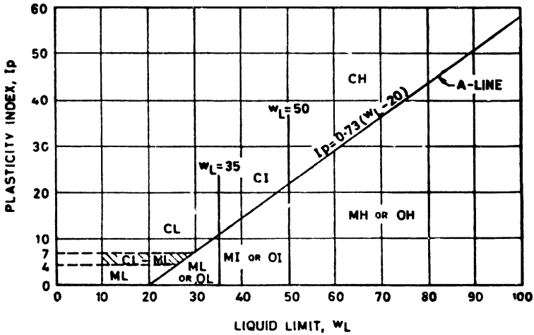
FIG. 1 PLASTICITY CHART
